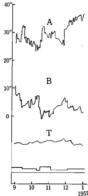
Fig. 6. Secular ground-tilting observed at Hondo (1956-1957).
