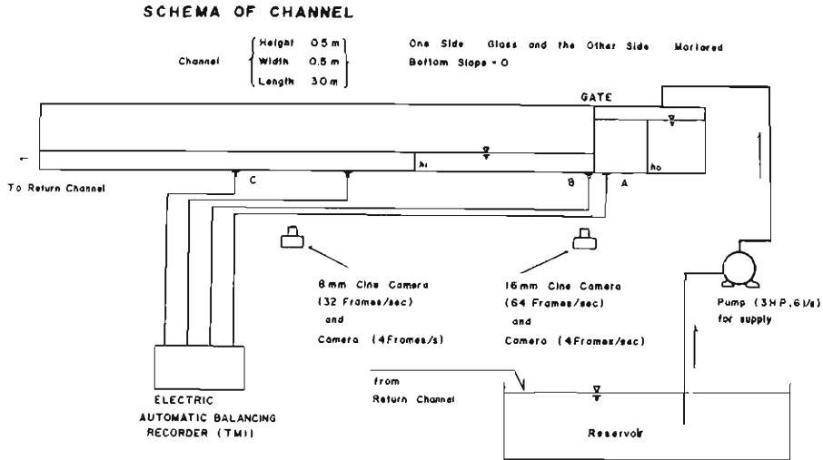
Fig. 1 Experimental apparatus.
