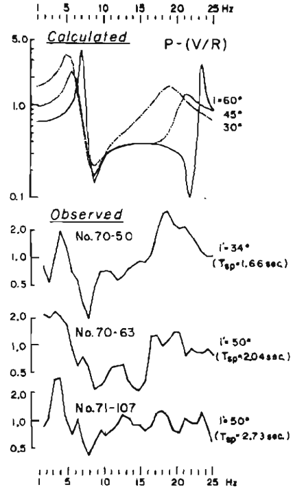
Fig. 6. Theoretical and observed spectral ratios of P waves. The parameters of the model are the same as those in Fig. 5.
