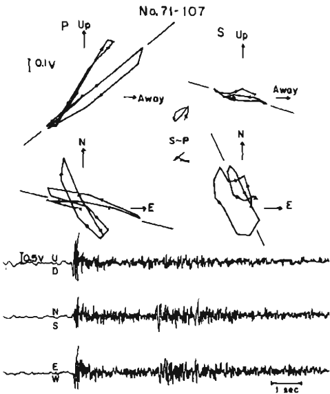
Fig. 3. The 25 Hz low-pass filtered seismograms and the particle motion diagrams of P, S-converted-P and S waves of the event with t_{s-p} of 2.73 sec.
