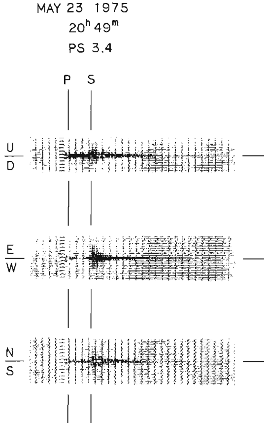
Fig. 20. Seismogram of the shock which originated in the Hamasaka region. Compare its waveform with that of the shock of October, 1971 shown in Fig. 18.
