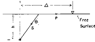
Fig. 17. Ray path of a SP wave.
