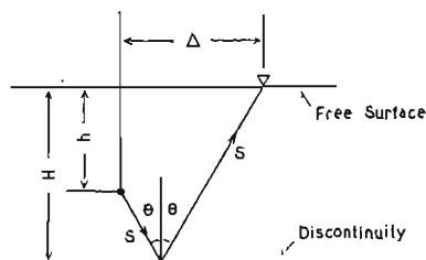
Fig. 10. Ray path for a SxS wave.
