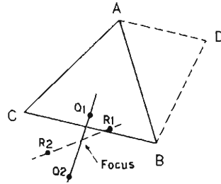
Fig. 25. Illustration of hypocenter determination for four stations.
