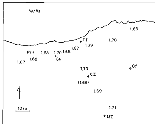
Fig. 7. Distribution of V_p/V_s . The parenthesized value is questionable.
