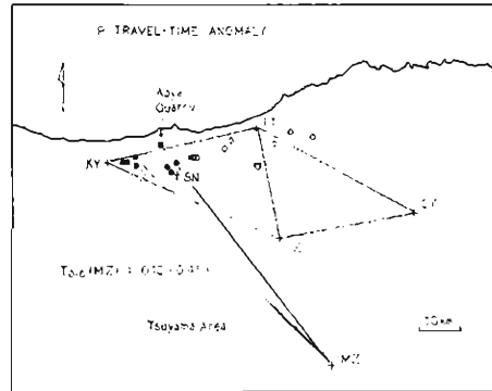
Fig. 4. Distribution of epicenters listed in Table 2. Solid circles indicate the events for which the anomaly in travel times was observed at MZ station and open circles mean the events which indicated no anomaly.
