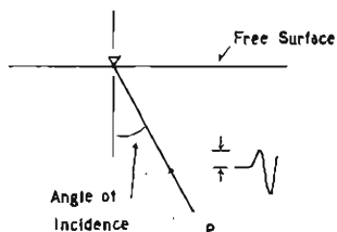
Fig. 9. Illustration of an angle of incidence.
