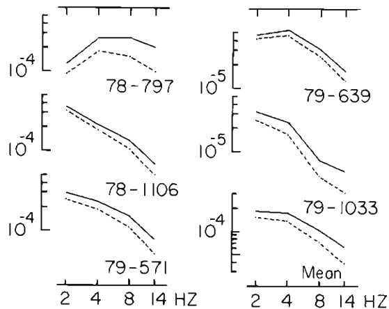
Fig. 12. The displacement spectral density of SH normalized to the hypocentral distance of 1 km, reduced by 2 for surface reflection. Q_s is given by 110 \sqrt{f} . The broken line represents the ones whose spectra are uncorrected for Q_s .
