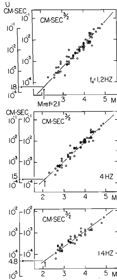
Fig. 5. Growth rate of the coda source factor with magnitude in each frequency band. Note that the source factor increases linearly with magnitude in the range of M=2.3\sim 4.9 . The scales for the source spectral density of the far-field shear wave at 1 km are added on the left side, which are obtained from the reference earthquake of M=2.1 in Fig. 12.
