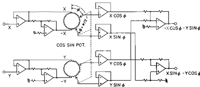
Fig. 8. Circuit diagram of the axis-transformer which generates the radial and transversal components from the two horizontal ones, N - S and E - W .
