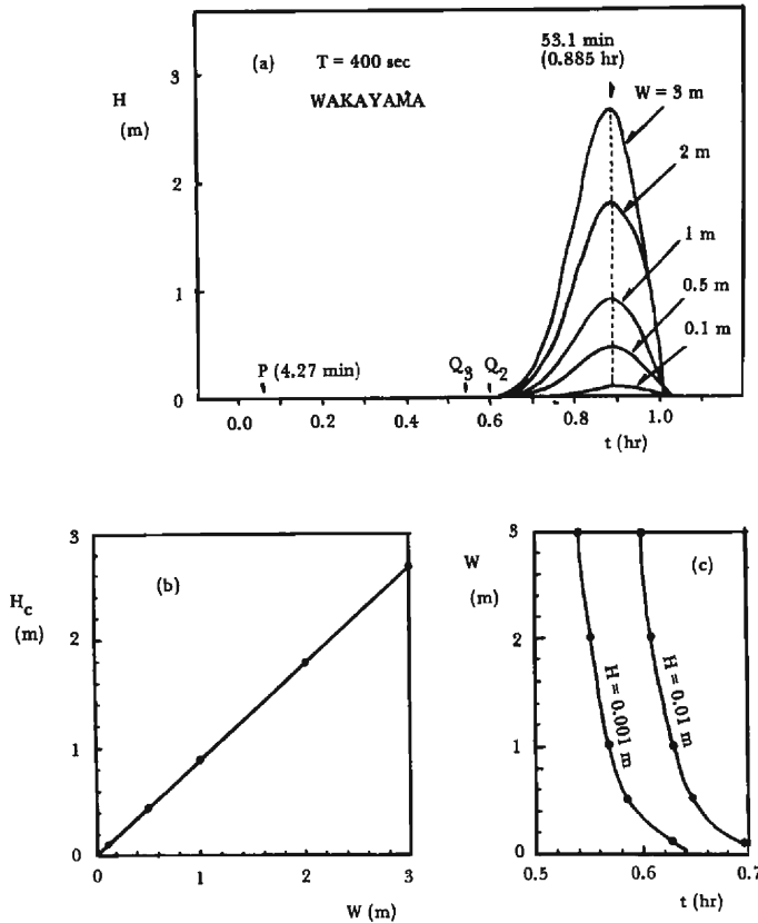
Fig. 4. Effect of initial disturbance W to the leading wave at Wakayama (a) wave patterns of the leading wave for T=400 \text{ sec} (b) relation between crest height H_c of the leading wave and initial disturbance W (c) arrival time Q_3 and Q_2 as a function of W (see text for detail)
