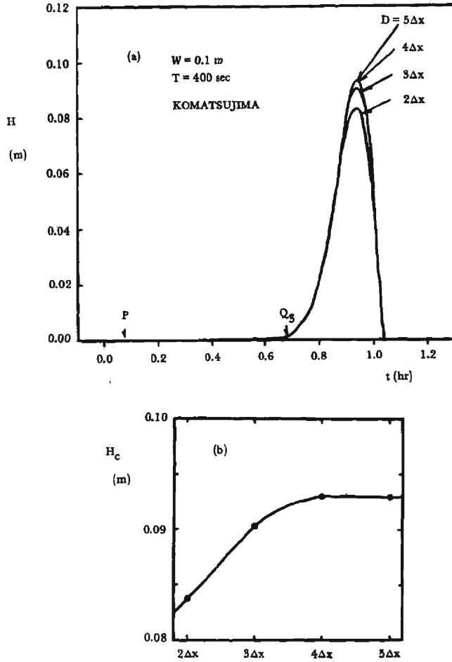
Fig. 5. Effect of length D of tsunami source to the leading wave at Komatsujima (a) wave patterns of the leading wave for T=400 sec and W=0.1 m (b) relation between crest height H_c of the leading wave and length D
