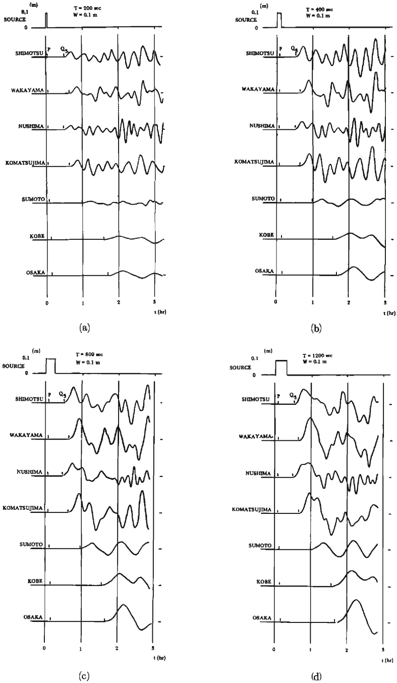
Fig. 2. Effect of duration time T to numerical tsunamis on the coast (scale of elevation at each station is the same as the scale for the source) (a) T=200 sec, (b) T=400 sec, (c) T=800 sec and (d) T=1200 sec
