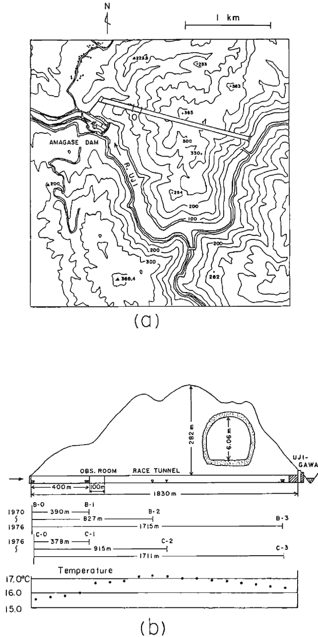
Fig. 1. Location map of the Amagase Observatory (a) and topographic profile along the observatory tunnel and positions of the station mark for electro-optical distance measurements and temperature distribution along the tunnel (b).
