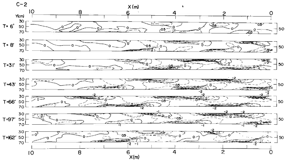
Fig. 14 Variation of the bed topography corresponding to the alternate bar development.
