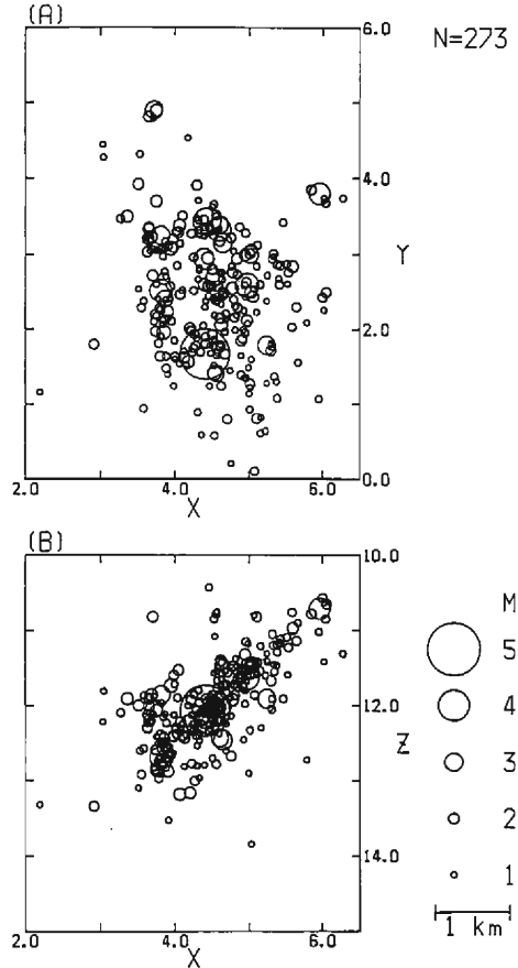
Fig. 4. Epicenter distribution (top) and depth distribution on the east-west vertical plane (bottom) of aftershocks with M 1.0 and greater (after Maeda (submitted)).
