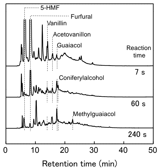
Fig. 4. HPLC chromatograms of the water-soluble portion from beech wood as treated for various reaction times in supercritical water at 380 °C/ 100 MPa .
