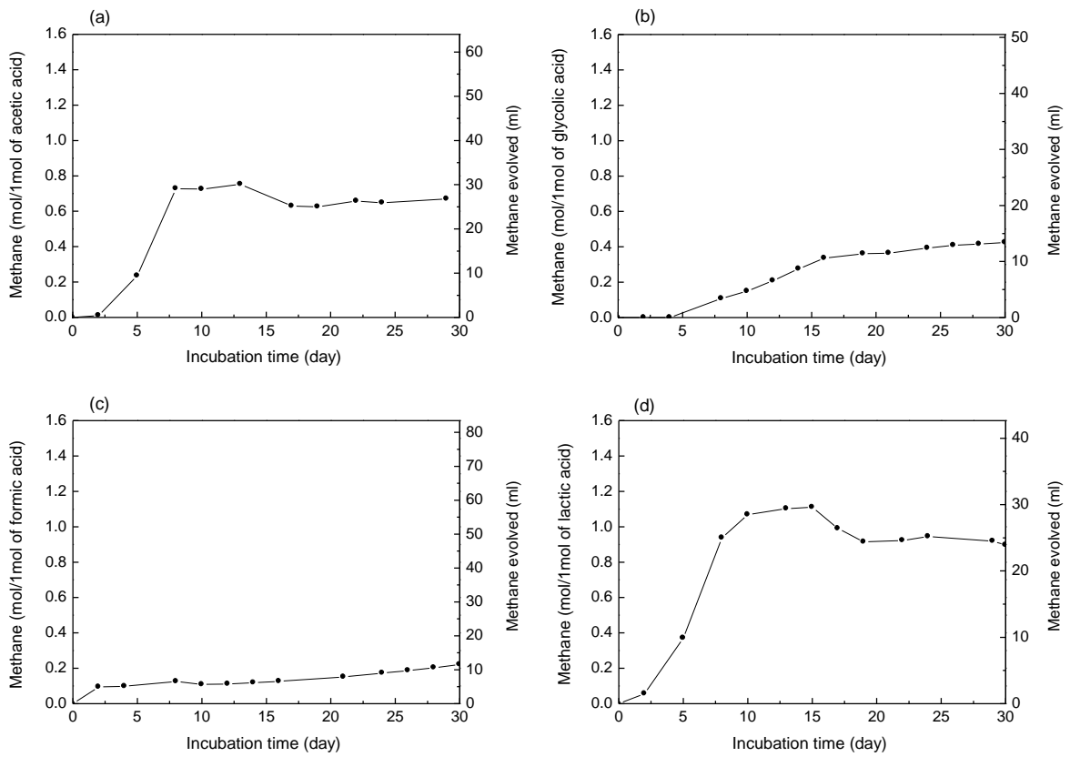
Fig. 2. Comparison of the methane production among various organic acids. (a) acetic acid; (b) glycolic acid; (c) formic acid; (d) lactic acid.
