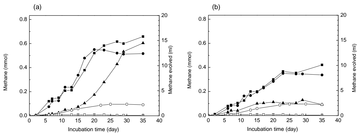
Fig. 3. Methane evolved from the water-soluble portion of beech wood as treated for various reaction times in supercritical water at 380 °C/ 30 MPa (a) and 380 °C/ 100 MPa (b). filled squares , treatment for 240 s; filled circles , treatment for 60 s; filled triangles , treatment for 7 s; open circles , untreated wood; open squares , only digested sludge
