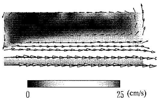
Fig. 12a Velocity vectors in the 2 nd embayment of the experimental flume measured by ECM
