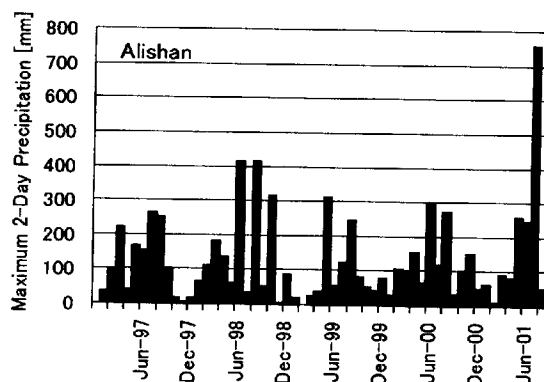
Fig.5 Amount of maximum two-days rainfall in each month at Alishan (January 1997~August 2001)
