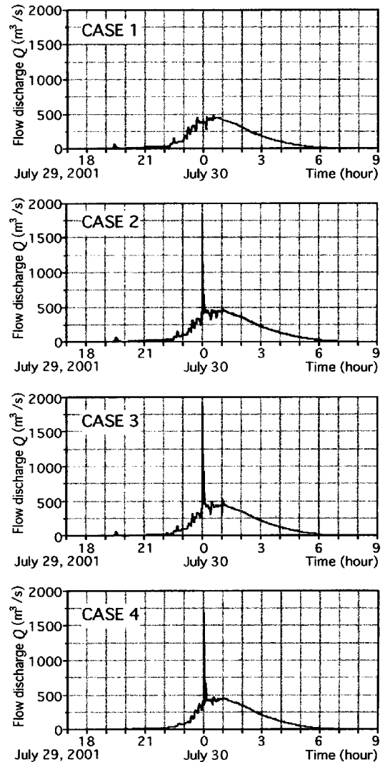
Fig.17 Temporal change of a flow discharge at the outlet of a ravine
