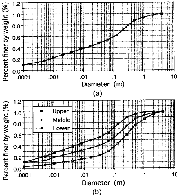
Fig.16(a) Grain-size accumulation curve used in the calculation (CASE 1~CASE 3)
