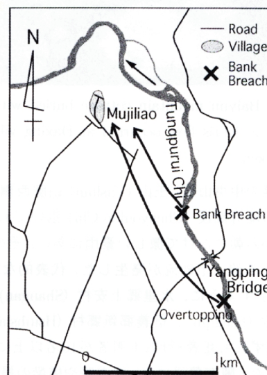
Fig.10 Overtopping and bank breach at Tungpurui Chi
