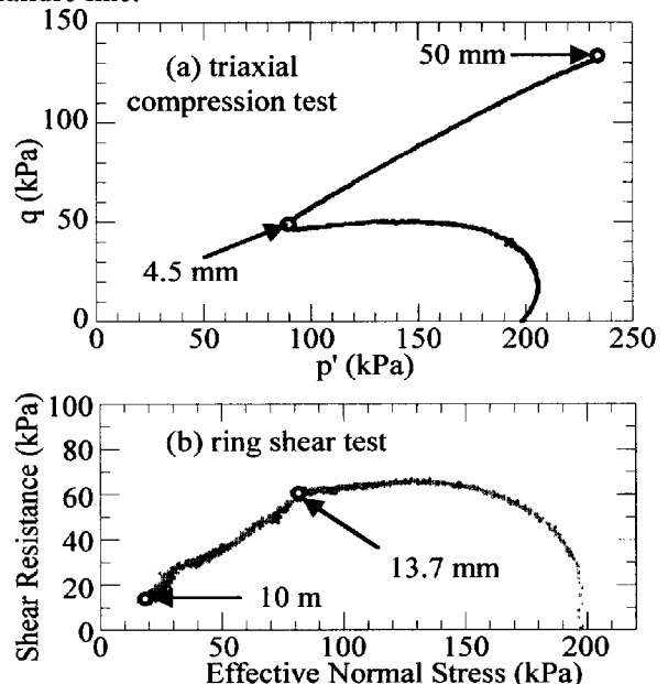
Fig. 3 Effective stress paths of loose silica sand no.8. (a)triaxial compression test (S 11 :e 0 =1.11), (b)ring shear test (S r1 :e 0 =1.10)
