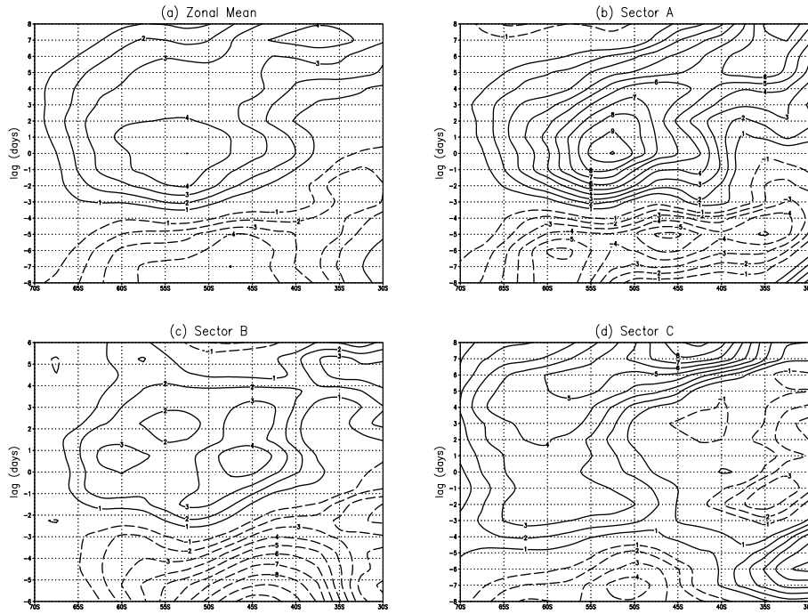
Fig. 17 Zonal averages of meridional component of \mathbf{E}_{uHFT} are calculated over (a) hemisphere or sectors (b)A, (c)B, and (d)C shown in Fig. 18. They are drawn on latitude-time sections. Solid and dashed contours indicate positive and negative anomalies, respectively. The contour interval is 1 \text{ m}^2 \text{ s}^{-2} , with the zero contour omitted.
