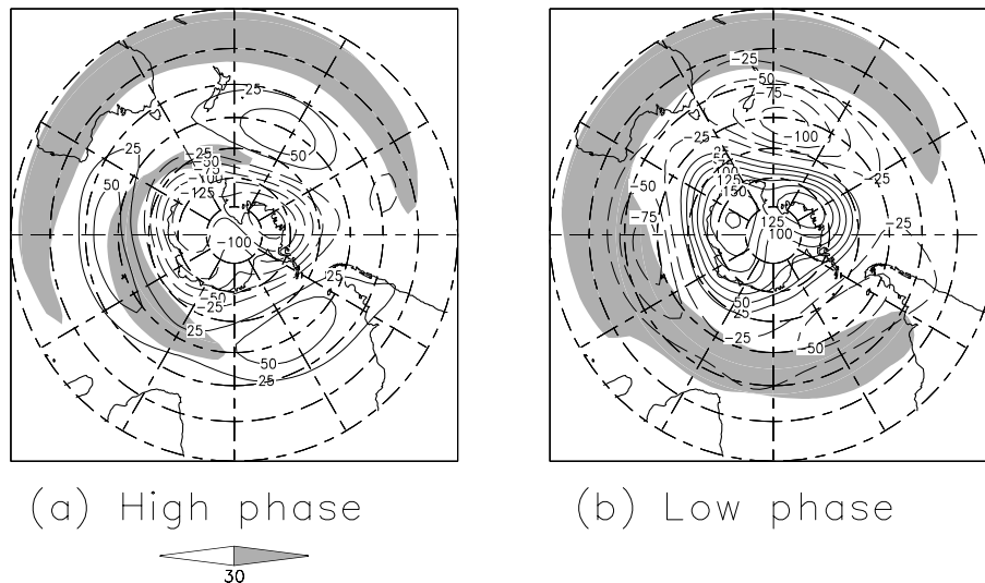
Fig. 3 Composite maps of the horizontal wind speeds and geopotential height anomalies on the 300-hPa surface for the cases when (a) the PC1 \geq 1 , and (b) the PC1 \leq -1 , respectively. Solid and dashed contours indicate positive and negative height anomalies, respectively. The contour interval is 25 m, with the zero contour omitted. The regions with wind speeds greater than 30 \text{ ms}^{-1} are shaded.
