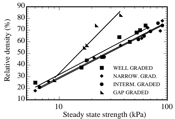
Fig. 5 Steady state strength of specimens confined within a normal stress range of 196 – 202 kPa
