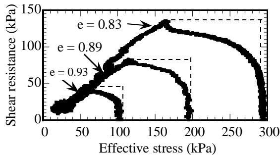
Fig. 12 Critical stress paths of Silica sand specimens
