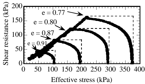
Fig. 11 Critical stress paths of Osaka sand specimens
