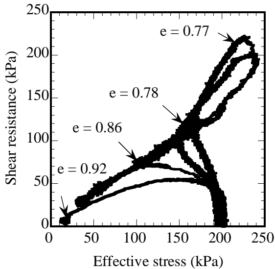
Fig. 14 Stress paths illustrating the influence of density on the behavior of silica sand materials
