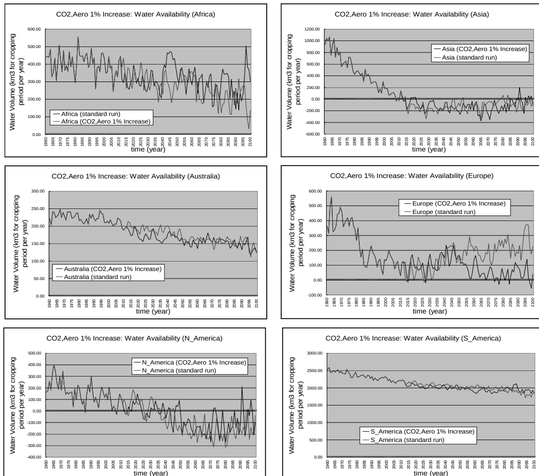
Fig. 11 Water Availability of 1% \text{CO}_2 Increase for Six Continents
