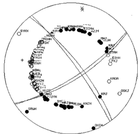
Fig.9 Focal mechanism solution from the polarities of P-wave first motions for the largest shock (M3.3) of the earthquake swarm on October, 2003 right beneath Hakusan Volcano.
