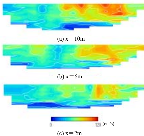
Fig. 8 Cross-sectional velocity distributions in several sections
