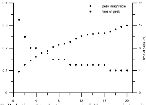
Fig. 9 Relationship between rainfall excess intensity to peak magntude of IUH and time of IUH peak
