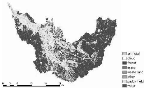
Fig. 7 Land cover classification of ASTER image
