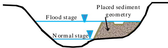
Fig. 12 Concept of sediment replenishment and placed sediment geometry on the bank of Nunome River.
