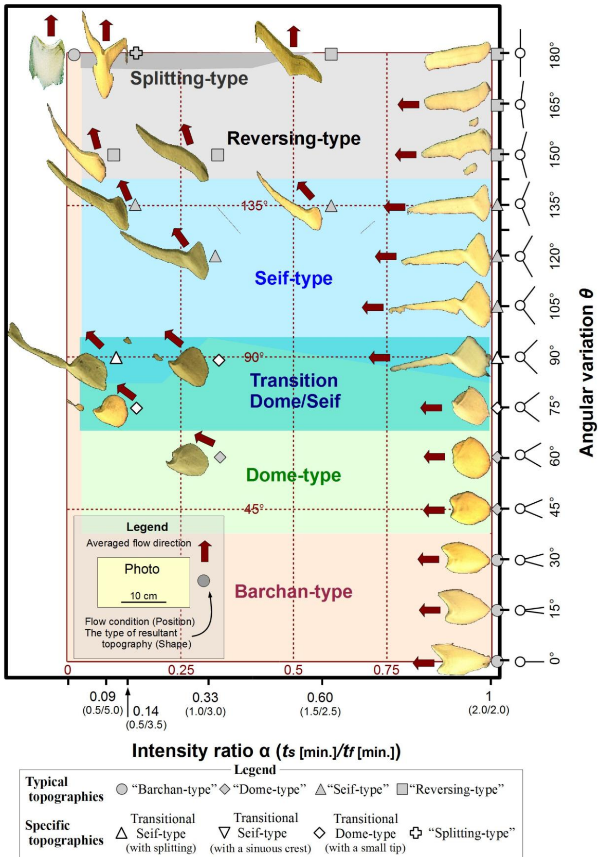
Fig. 2 A phase diagram of the shape of isolated san topographies under bidirectional flow conditions between the angular variation \theta and intensity ratio \alpha .
