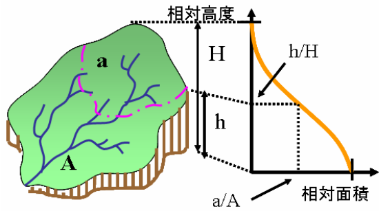
Fig. 2 Hypsometric curve
