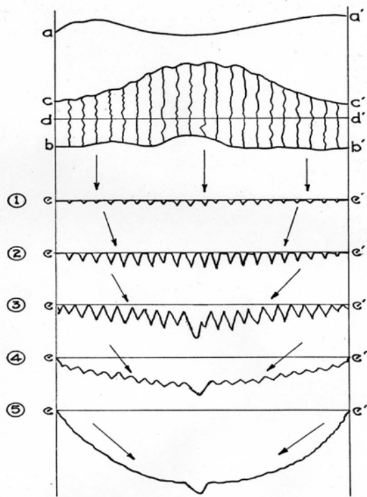
FIGURE 22.—Development of a valley by cross-grading
