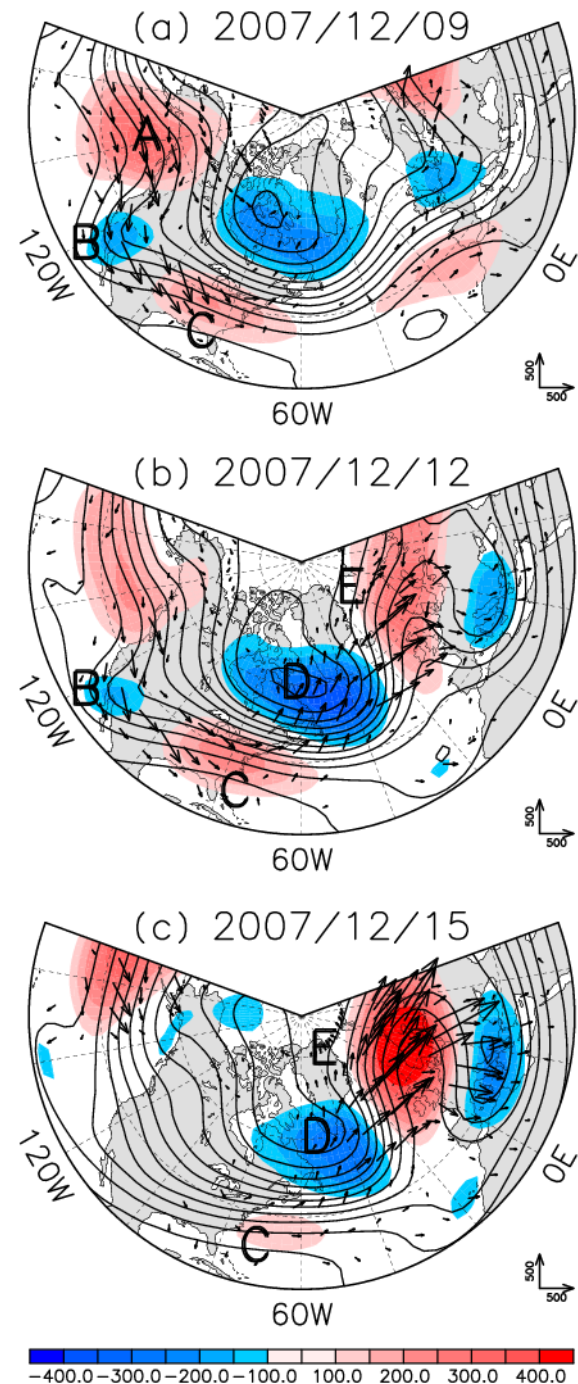
Fig. 1 Time evolution of 5-day mean 300-hPa height fields (contour interval: 120 m), anomalous fields (color shade), and the wave activity density flux (arrows: the reference arrow is 500 \text{ m}^2/\text{s}^2 ) defined by Takaya and Nakamura (2001). (a) 9 Dec. (b) 12 Dec. (c) 15 Dec. 2007.
