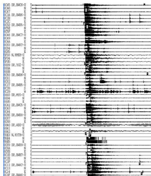
Fig.9 Examples of waveforms of a micro earthquake (2009.1.23).
