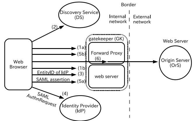
Figure 2. Flow of federation proposed proxy
