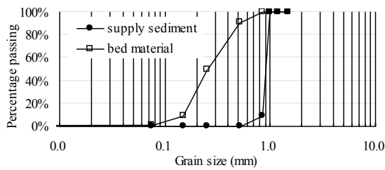
Fig.2 Grain size distribution of bed material and supplied sediment in the experiment
