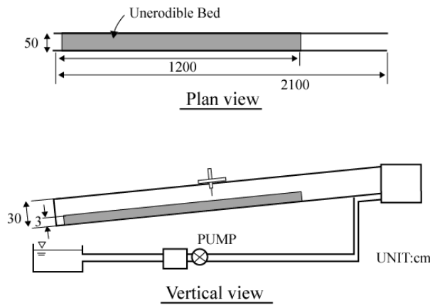
Fig.1 Experimental flume
