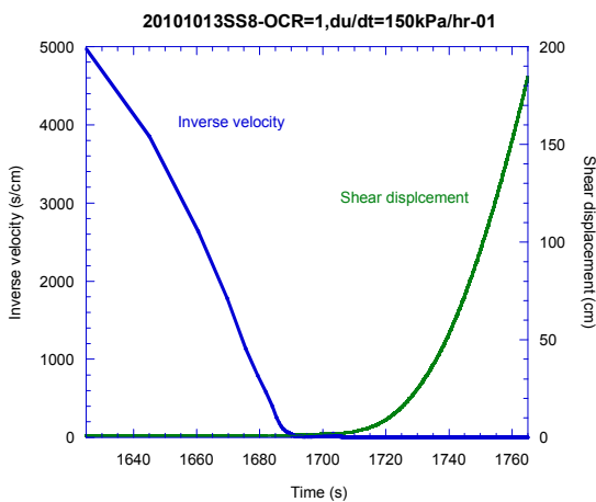
Figure 6: Inverse velocity and shear displacement at final stage of Tertiary creep
