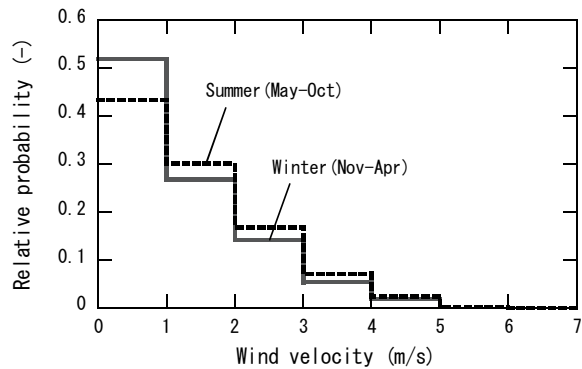
Fig.6 Frequency of wind velocity in Kyoto city.
