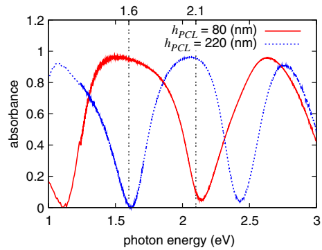
Fig. 2. (Color online) Spectrum comparison of local plasmon resonator chips whose PCL thicknesses are h_{\text{PCL}} = 80 and 220 \text{ nm} .
