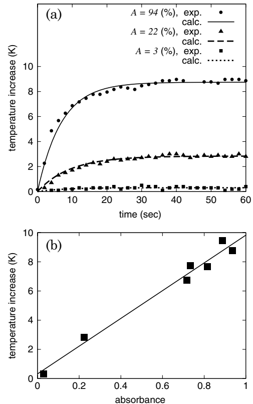
Fig. 3. Photothermal properties of local plasmon resonators. (a) Trace of the temperature increase of the water in the cell. Both measured and calculated (solid curves) distributions are shown. (b) The temperature increase of the water in the cell at equilibrium as a function of the optical absorbance. The solid line represents a linear fit, where Q = 8.4 (\text{mW/K}) .
