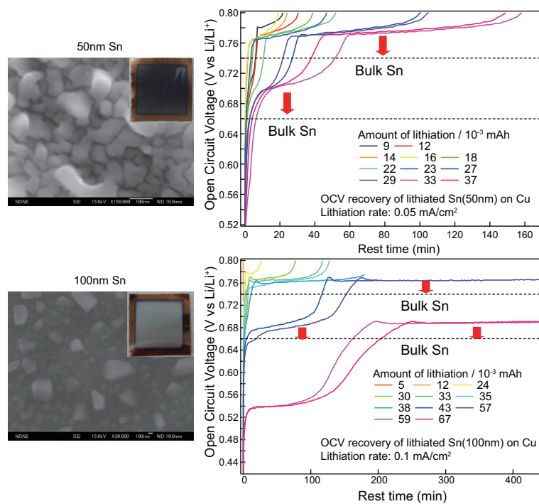
FIG. 5: The OCV-RT curves measured for the Sn thin films with 50 nm and 100 nm thicknesses (the deposited area is 9 \text{ mm} \times 9 \text{ mm} in the both cases) on Cu substrates prepared by the sputtering method. The FE-SEM micrographs are also shown, from which almost nanoparticles are formed on the substrate in both cases. The OCV behavior that is going to increase over 0.8 V may be caused by the reaction with the Cu substrate or Sn-Cu compound which seems to be formed near the substrate surface.
