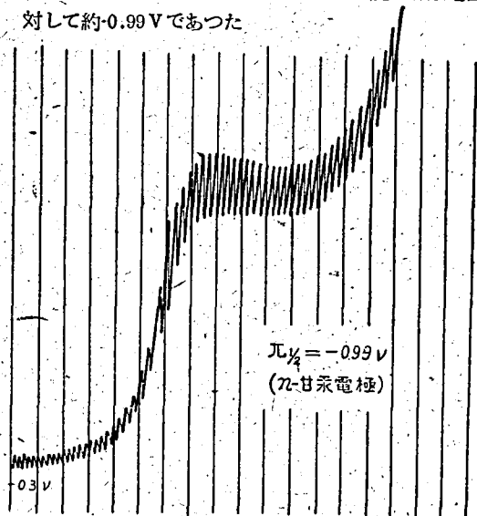
Fig 2. Polarogram of \alpha -Hepta.
