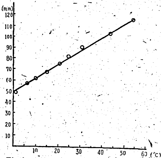
Fig 1. Effect of temperature on the wave height of \gamma -BHC.
