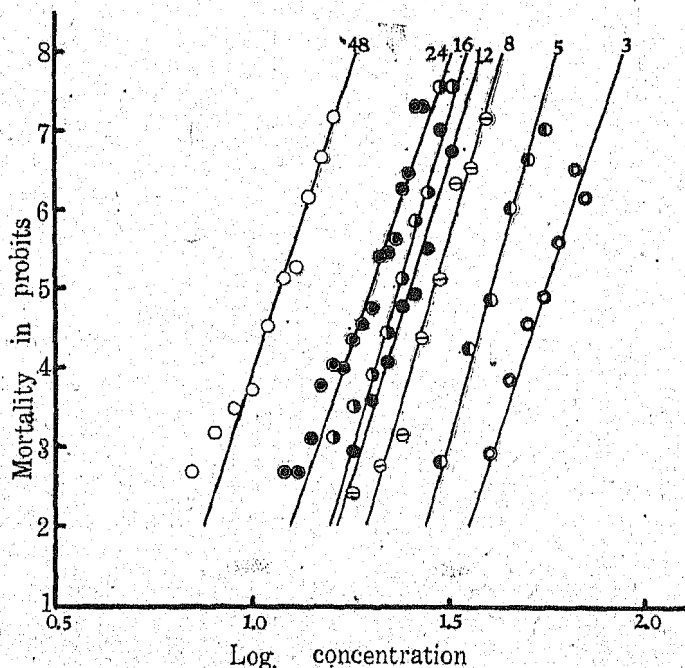
Fig. 2. Concentration-mortality curves measuring the toxicity of carbon disulfide to the rice weevil in terms of mortality in probits and log-concentration at seven different exposure times (3, 5, 8, 12, 16, 24, and 48 hours).
