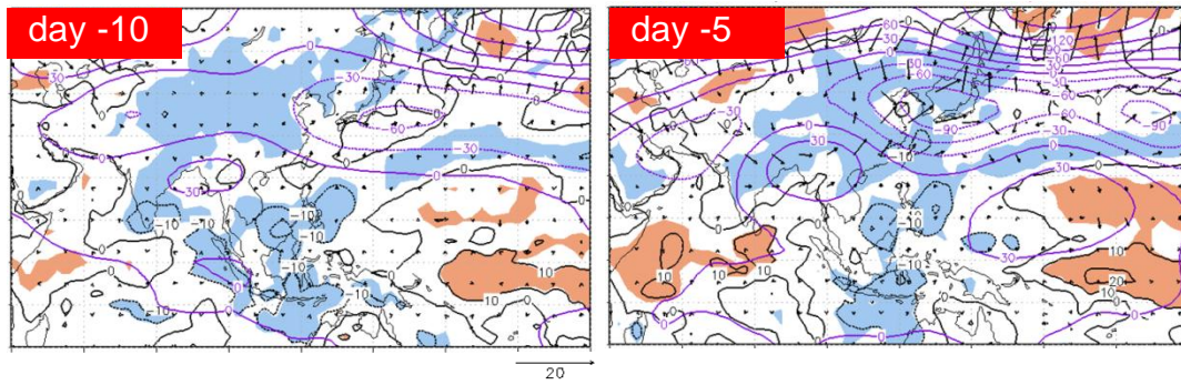
Fig. 8 As in Fig. 7 except for the anomaly of OLR (black contour; W/m^2 ) and 250-hPa stream-function ( \times 10^5 m). Regions with a statistical significance over 99% for OLR anomaly are color shaded.
