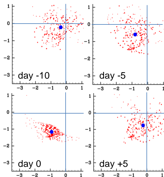
Fig. 6 Time evolution of the observed sample data residing in the vicinity of the point O : (PC1, PC2)=(-1.0, -1.4) at day 0 in the 2D phase space. Blue dots indicate their centroids.
