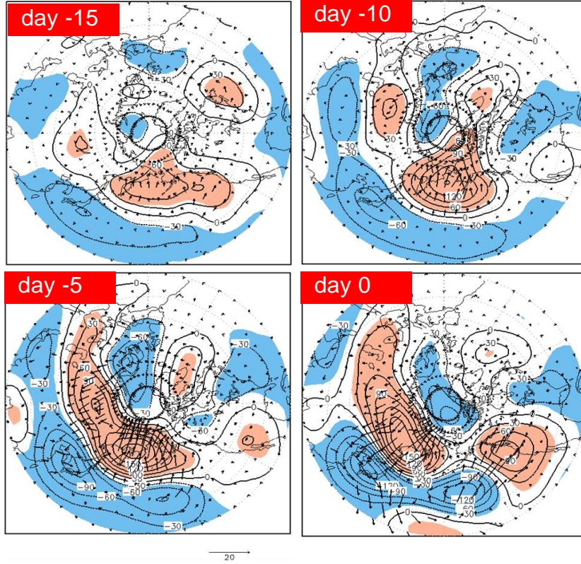
Fig. 7 Compositing anomaly of 250-hPa geopotential height anomaly (m) corresponding to green dots in Fig.5. Contour interval is 30m, and regions with a statistical significance over 99% are color shaded. The arrows indicate wave-activity flux ( \text{m}^2/\text{s} ) of Takaya and Nakamura (1997).
