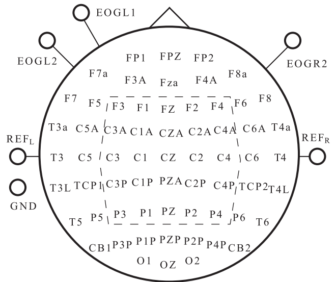
Fig.2 Arrangement of electrodes. Reference electrodes were placed on the right and left earlobes (REF R , REF L ) and the grounded electrode (GND) was placed on the left mastoid. EOGL1, EOGL2, EOGR2, and FP1 were EOG electrodes: FP1 was also used as an EEG electrode. The squares show the region for classification. Electrodes, which are used by CSPs, are surrounded with a dashed line.
