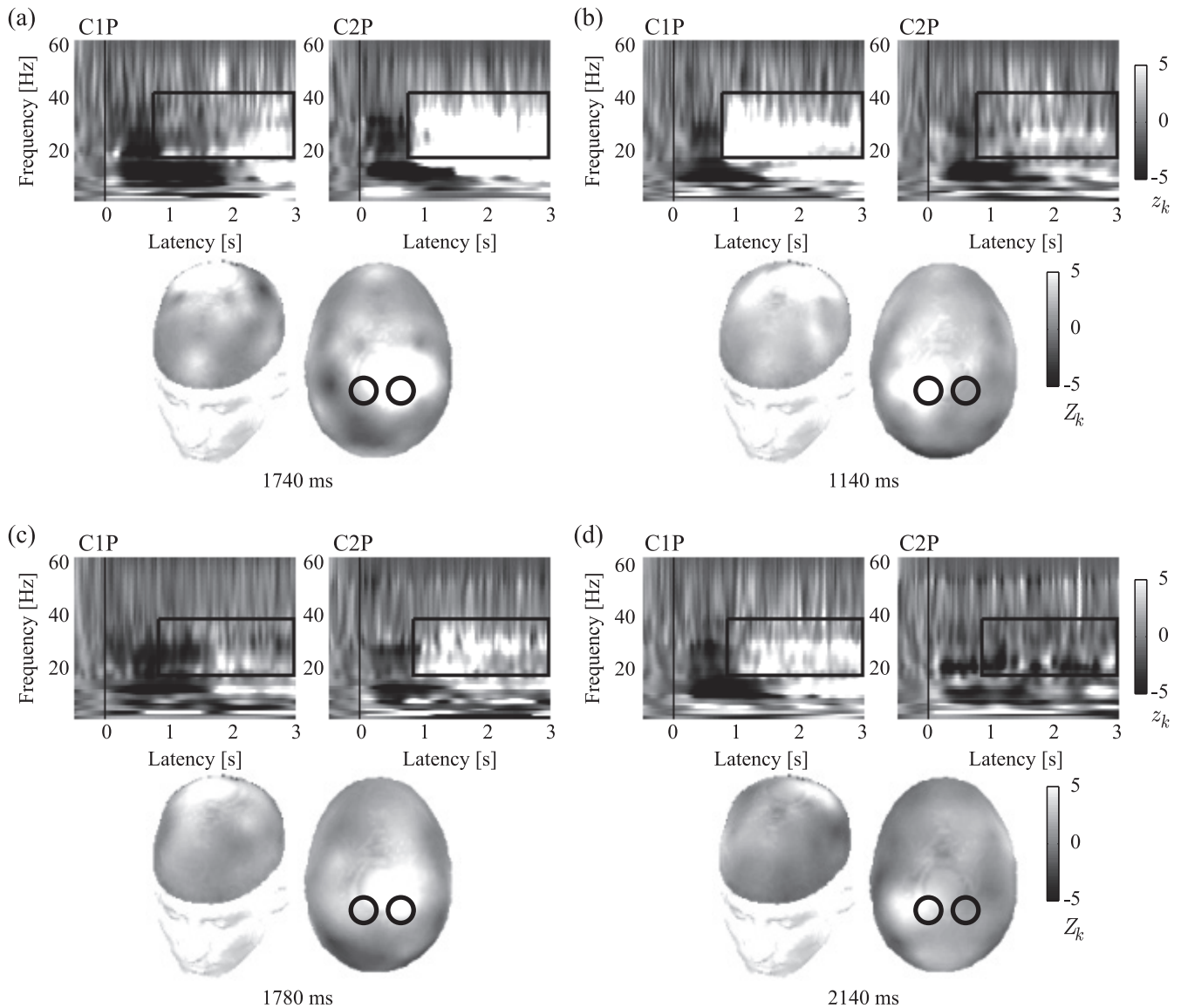
Fig. 4 Time-frequency maps [z_k(t, f)] and the topography of Z_k(t; f_L, f_H) at the peak latency in the condition of (a) left-hand movement, (b) right-hand movement, (c) left-hand-movement imagery, and (d) right-hand-movement imagery in subject 1. The range of latency and frequency for classification is surrounded by a black rectangle. Channels C1P and C2P are each surrounded by a black circle.
