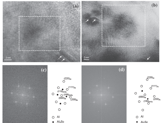
Fig. 11 TEM images of Al 3 Sc precipitates in the 300°C Aged-ARB specimen after 9 cycles of ARB. (a) precipitates having the identical orientation relationship with matrix and (b) precipitates with different orientation relationship with matrix. (c) and (d) are corresponding diffraction patterns obtained by FFT analysis for the areas surrounded by white-broken lines in (a) and (b), respectively.
