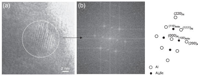
Fig. 13 High-resolution TEM images of \text{Al}_3\text{Sc} precipitates formed at 400°C for 10Ks and then deformed by ARB up to 9 cycles. (a) A coherent precipitate (surrounded by dotted circle), and (b) corresponding Fourier analyzed pattern for (a).
