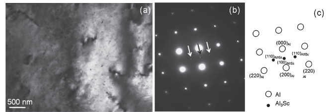
Fig. 10 TEM micrographs of the 300°C Aged-ARB specimen after 1 cycle ARB process. (a) TEM microstructure, (b) SAD pattern and (c) a key diagram.
