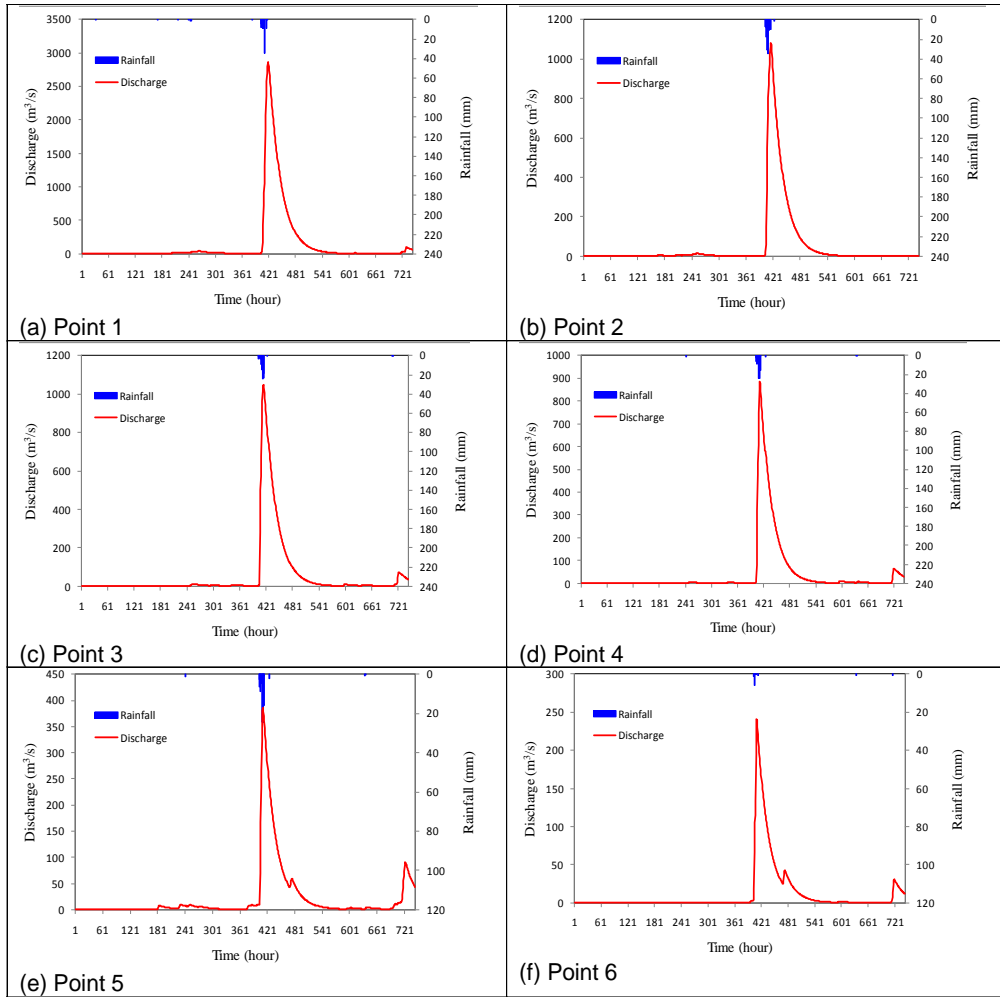
Fig. 7 Simulation of flash flood event of (Jan.18-22, 2010) at several sub-catchment outlets of Wadi El-Arish: a) Point 1, b) Point 2, c) Point 3, d) Point 4, e) Point 5, and f) Point 6.
