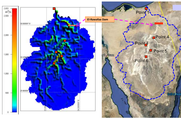
Fig. 8 Distribution maps of discharge of Jan. 2010 flash flood event at Wadi El-Arish, Sinai Peninsula, Egypt, showing discontinuous flow of discharge (red marks are the position of sub-catchments outlets of simulation).
