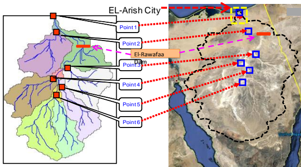
Fig. 6 Wadi El-Arish catchment, Sinai Peninsula, Egypt, in squares the target outlets for flash flood simulation and the location of El-Rawafaa Dam.
