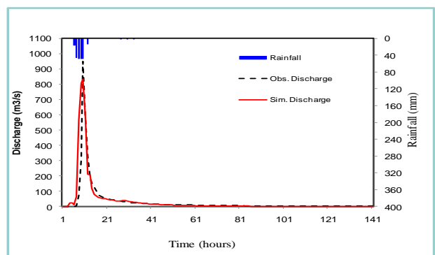
Fig. 4 Model calibration and validation at wadi Al-Khoud, Oman, during the event of (Mar.18, 2007) 11
