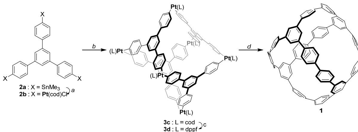
図 1. かご状三次元 \pi 共役系化合物の合成。 Reaction conditions and reagents: a) Pt(cod)Cl 2 (3.0 equiv), 1,2-Dichloroethane, 50 °C/20 h, 82%. b) 2a (1.0 equiv), 1,2-Dichloroethane, 50 °C/30 h, 81%. c) dppf (6.0 equiv), CH 2 Cl 2 , rt/19 h, 86%. d) XeF 2 (6.0 equiv), toluene, 90 °C/20 h, 12% (4steps from 2a).
