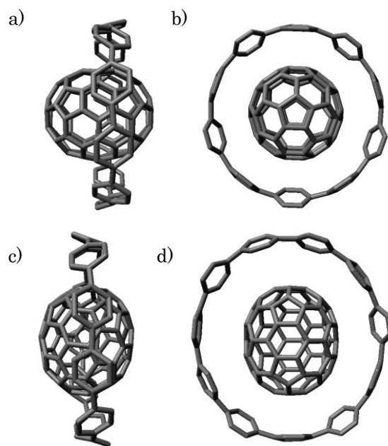
Figure 2. Optimized structure of a) [10]CPP \supset C 70 , b) [10]CPP \supset C 70 (top view), c) [11]CPP \supset C 70 and d) [11]CPP \supset C 70 (top view) at the M06-2X/6-31G* level of theory.
