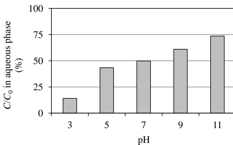
Fig. 4. 2. 9 nC_{60} adsorption on activated sludge as a function of pH.
