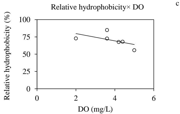
Fig. 4. 2. 13 \zeta potential (a), size (b) and relative hydrophobicity (c) of the activated sludge as a function of SRT, HRT and DO.
