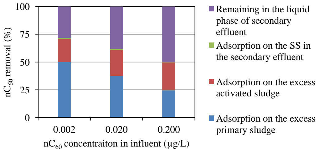
Fig. 6. 4 Contribution of each unit on the nC 60 removal in the activated sludge process at different initial nC 60 concentrations. Condition as follows: SS 0 0.15 g/L; R SS 70%; HRT 8 h; SRT 15 day; MLVSS 2 g/L; nC 60 0.002, 0.020, and 0.200 µg/L.
