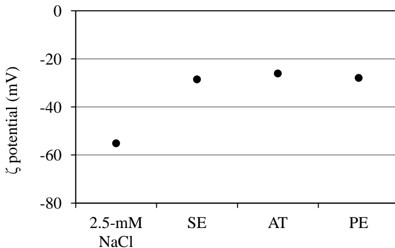
Fig. 4. 1. 4 \zeta potential of nC 60 in water samples. PE: primary effluent; AT: aeration tank liquor; SE: secondary effluent
