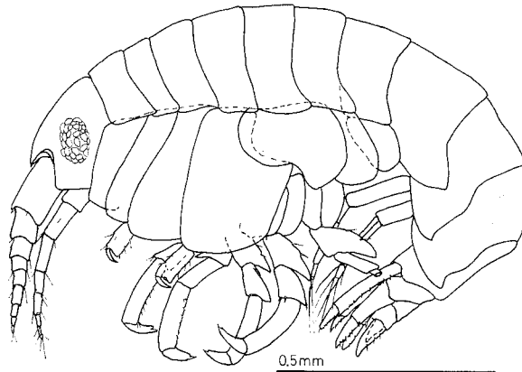
Fig. 269. Dactylopleustes obsolescens sp. nov. Holotype, male (?), 2.0 mm.
