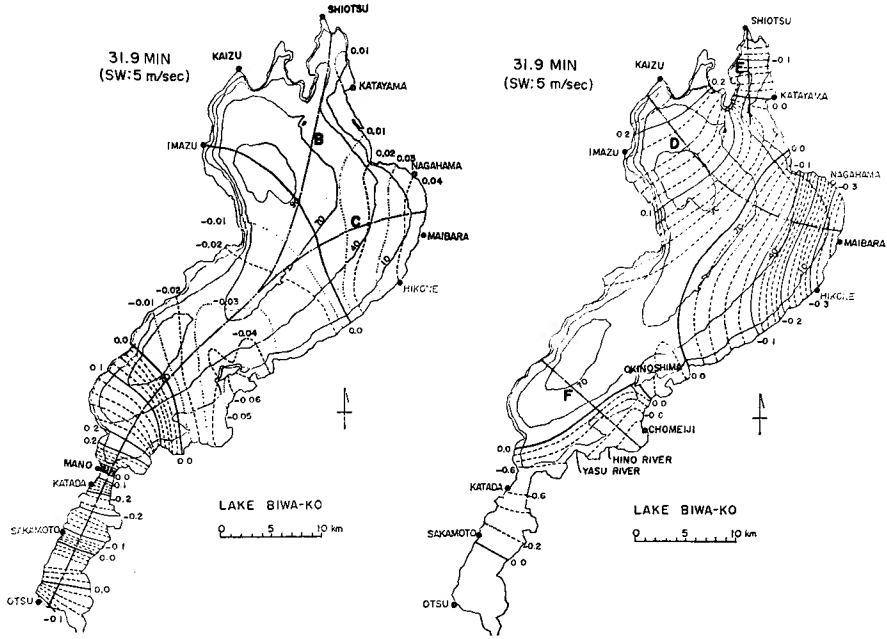
Fig. 4. Horizontal distributions of the amplitude of the seiche with the period 31.9 minutes in the case SW; (a) for the longitudinal seiche (left side), and (b) for the lateral seiches (right side).
