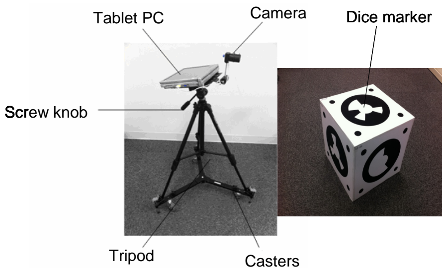
Fig. 4.11: Appearance of verification subsystem.
