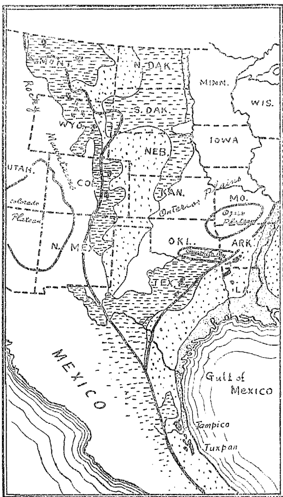
Tertiary Mesozoic. Paleozoic. Quaternary Topographic boundary Oil fields.
