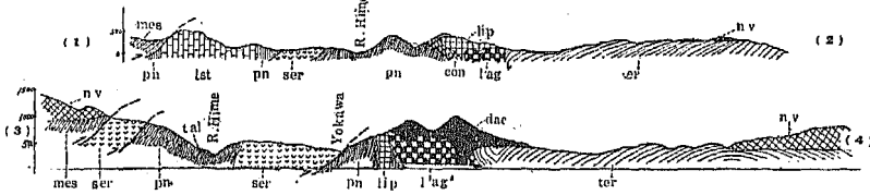
GEOLOGICAL PROFILE
