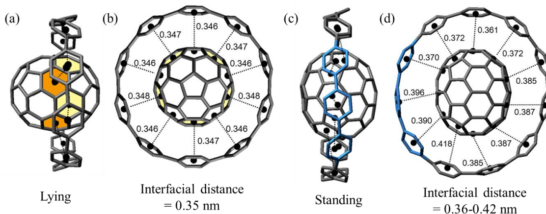
Figure 1. Optimized structure of a) C_{70}\subset[10] CPP, b) C_{70}\subset[10] CPP (top view), c) C_{70}\subset[11] CPP and d) C_{70}\subset[11] CPP (top view) at the M06-2X/6-31G* level of theory. Numbers indicate the interfacial distances (nm), defined by the distance between the centroids of phenylene units of CPP and the nearest centroids of a hexagon or pentagon of C_{70} .
