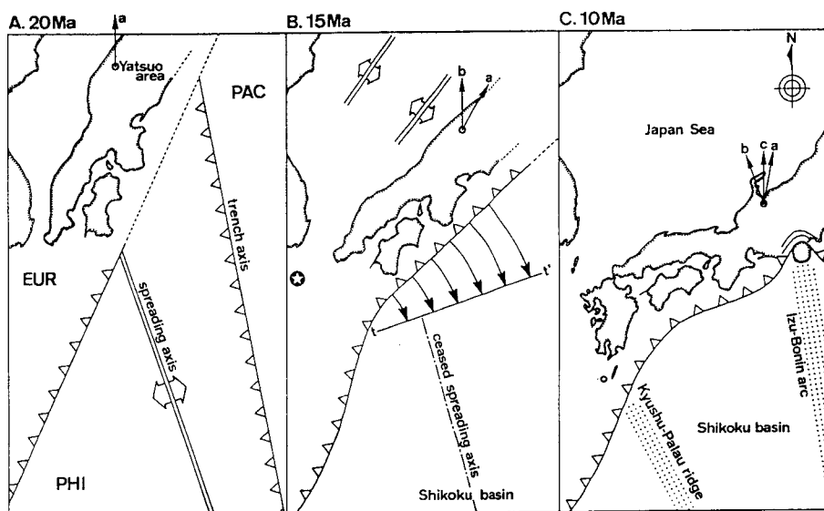
Fig. 11. Schematic reconstruction around Southwest Japan before, during and after the back-arc opening of the Japan Sea in middle Miocene. A: Pre-opening stage (20 Ma). Paleopositions of Southwest Japan and the plate boundary are adapted from OTOFUJI & MATSUDA (1987) and SENO & MARUYAMA (1984), respectively. EUR=Eurasia plate; PAC=Pacific plate; PHI=Philippine Sea plate. B: Opening stage (about 15 Ma). Southwest Japan is rotating clockwise associated with rapid hinge rollback of the downgoing Philippine Sea plate. t-t' shows the final position of hinge. Star represents the pivot of rotation (OTOFUJI & MATSUDA, 1987). C: Post-opening stage (10 Ma). Differential rotations within Southwest Japan raised by the collision of the Izu-Bonin arc have already finished, too. Arrows a and b show horizontal components of paleomagnetic directions in the lower and uppermost part of the Yatsuo Group, respectively. Arrow c corresponds to paleomagnetic data in the Tonami Group acquired after the clockwise and counterclockwise rotations of the Yatsuo area.
