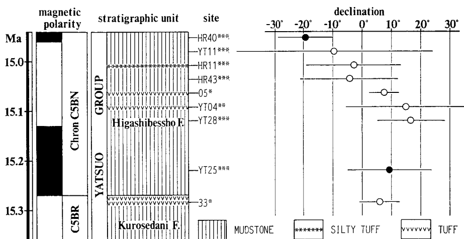
Fig. 5. Enlargement of Fig. 4 around 15 Ma. Magnetostratigraphy of the Yatsuo Group is after ITOH & HAYAKAWA (1988). Stratigraphic positions of the paleomagnetic data within a normal or reversed polarity interval are proportional to the thickness of the sampled section.
