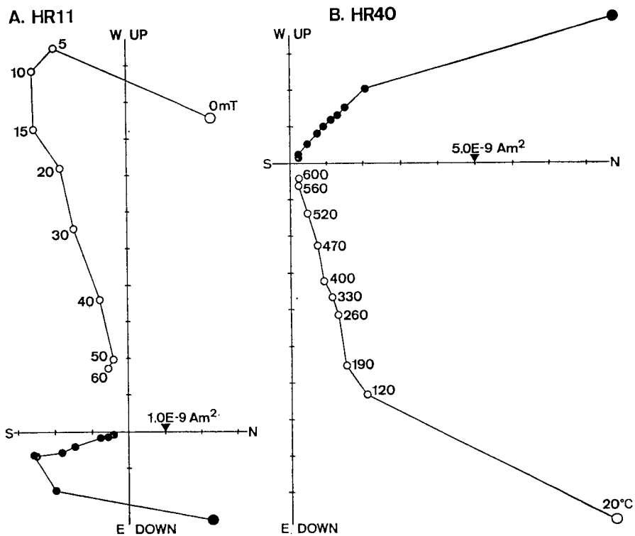
Fig. 3. Typical vector-demagnetization diagrams of progressive alternating field (A) and thermal (B) demagnetization tests for sedimentary rocks obtained from the Yatsuo area. Solid (open) circles are projection of vector endpoints on the horizontal (N-S vertical) plane in in-situ coordinates. Unit of coordinates is bulk remanent intensity. Numbers attached to symbols are demagnetization levels in mT or °C. Progressive change of vector endpoints shows a straight trend indicating stable magnetization.
