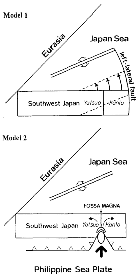
Fig. 7. Two models for the mechanism of the differential rotation as confirmed by paleomagnetic data in the Yatsuo area. (Model 1) Left-lateral shear is produced on the margin of a rotating arc, resulting in counterclockwise rotation of the Yatsuo and Kanto areas. (Model 2) Landmasses on the Philippine Sea plate collide against the Japan arc, resulting in counterclockwise rotation of the Yatsuo area and clockwise rotation of the Kanto area.
