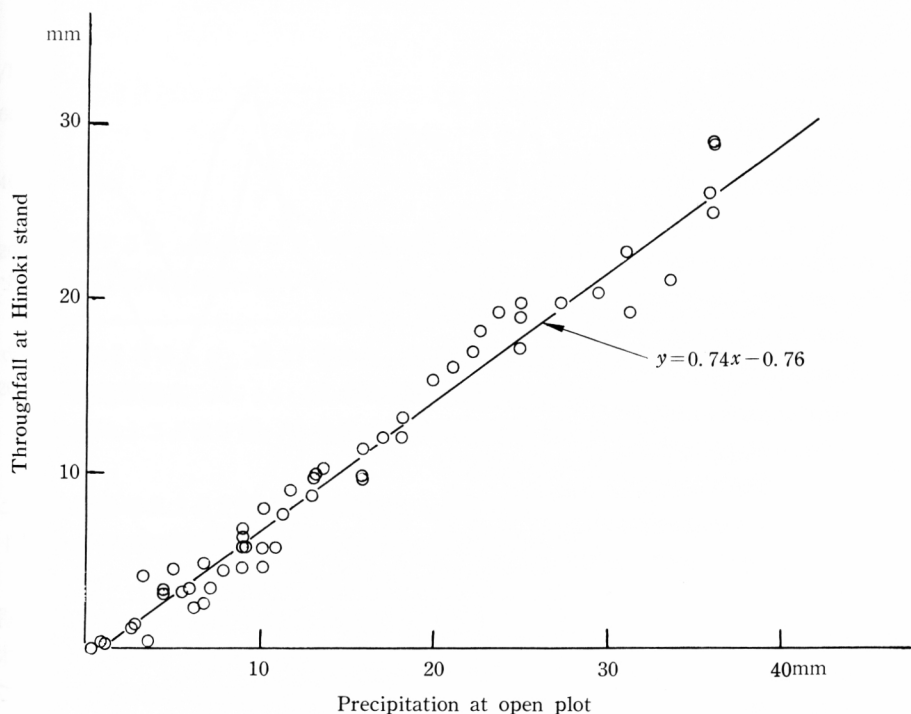
第3図の1 林外雨量とヒノキ林内雨量の関係 Fig. 3-1 Relationship between precipitation at open plot and throughfall at Hinoki stand.
