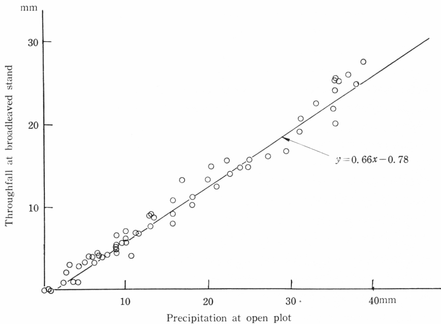
第3図の2 林外雨量と広葉樹林内雨量の関係 Fig. 3-2 Relationship between precipitation at open plot and throughfall at broad leaved stand.
