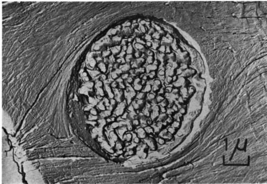
Fig. 7. Bagtikan ( Parashorea plicata ). A replica of the surface of a vessel, showing the surface view of a vestured pit.
