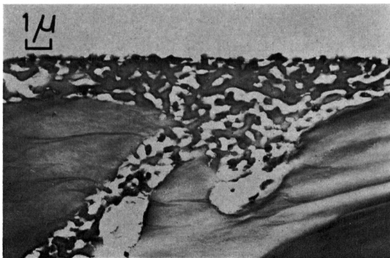
Fig. 11. Bagtikan ( Parashorea plicata ). A transverse section of vestured pit between a vessel and a tracheid, showing the vesture existed in vessel pit and on the vessel wall.
