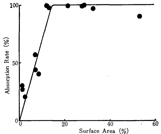
Fig. 1. Rate of CO 2 absorption as a function of surface area of alkaline solution. Abscissa: percent of the base area of the container. Ordinate: percent of the maximum rate of absorption.
