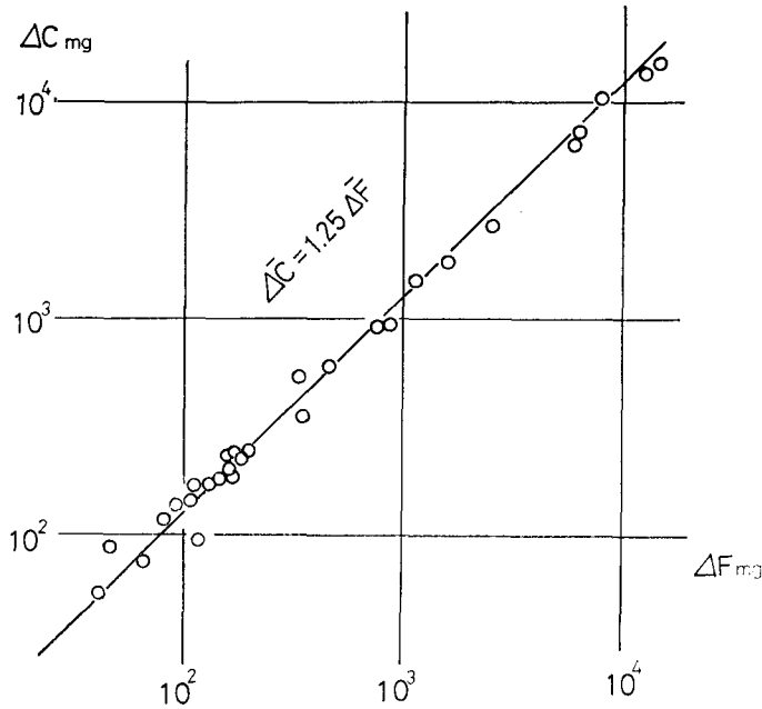
Fig. 2. Relationship between food consumption ( \Delta\bar{C} ) and defecation ( \Delta\bar{F} ) during a certain unit of time (20 days).
