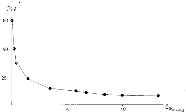
Fig. 7. Food consumption of the pine caterpillar population.
