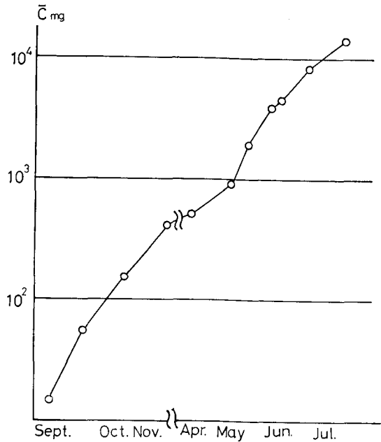
Fig. 1. The cummulative amounts of food consumption ( \bar{C} ) by and individual larva.
