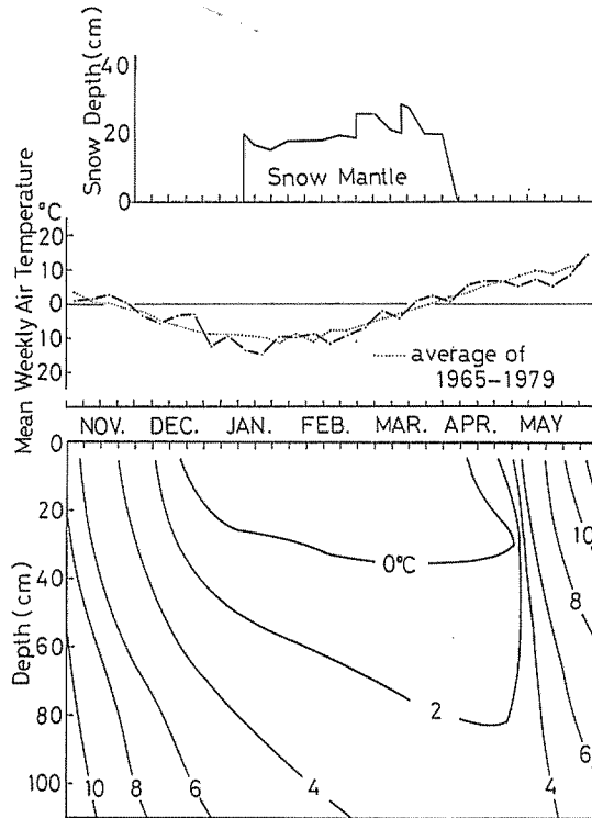
Fig. 2 Penetration of cold and warm into the ground in the winter of 1980-1981
